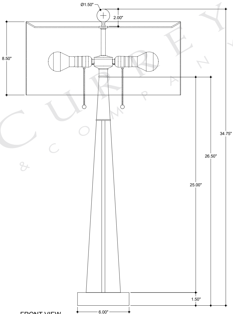
FRONT VIEW
