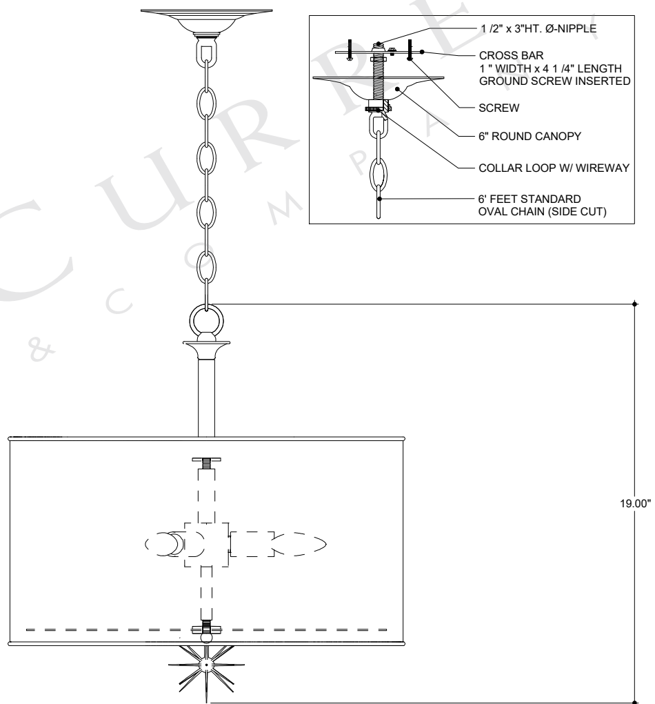
FRONT VIEW
