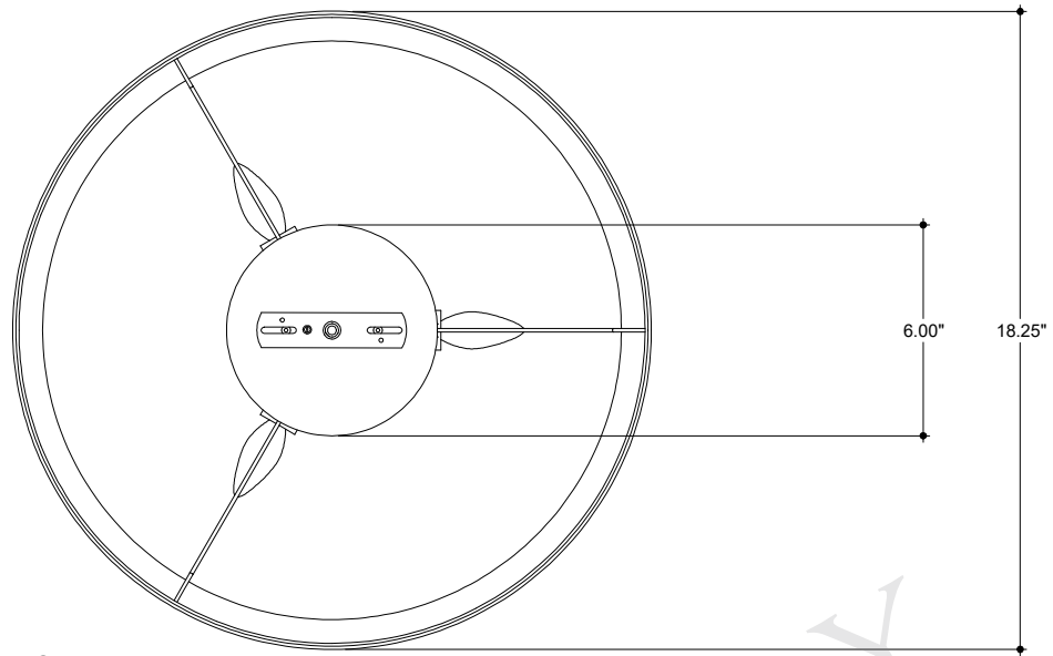
TOP VIEW
