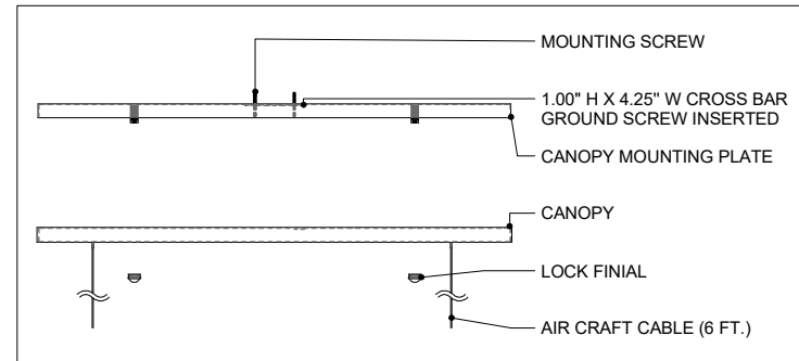
CANOPY DETAIL
